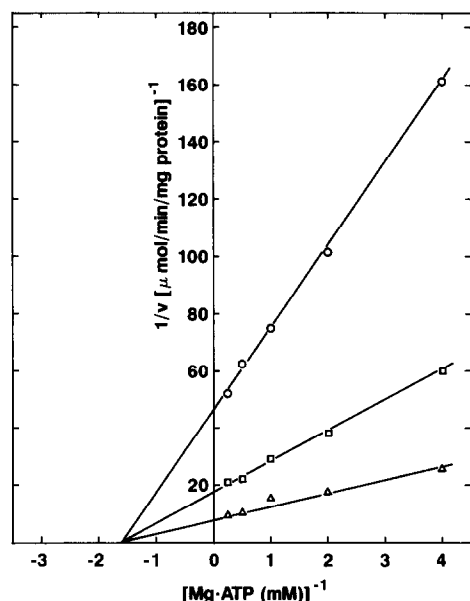
Fig.2. Double reciprocal plots of the \text{Na}^+ -stimulated ATPase activity. Cells were grown on KTY medium containing 0.2 M NaCl at pH 6.0 ( \circ ), at pH 7.5 ( \square ) and at pH 9.5 ( \Delta ). Preparation of the cell membranes and the assay of ATPase activity were performed as described in section 2. The \text{Na}^+ -stimulated ATPase activity was determined by B-A as shown in table 1. The ratio of \text{ATP}:\text{Mg}^{2+} was kept constant at 1.
